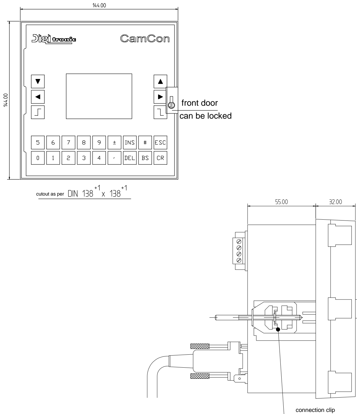
Fig.: Drawing to help with the installation of the CamCon Terminal
