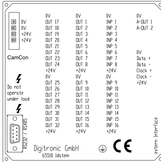
Fig.: Rearview of the CamCon Terminal with pin allocation
